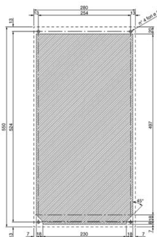
SEMI-FLUSH MOUNTING
