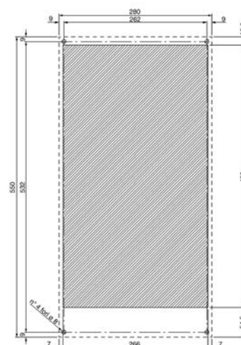
EXTERNAL MOUNTING
